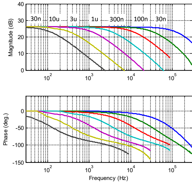
Figure 4. Small signal frequency response
