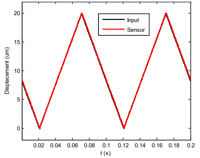
Figure 9. 10-Hz Full-Range Tracking Performance
