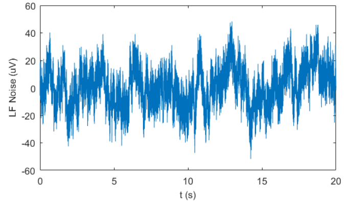
Figure 5. Low frequency output noise (0.03 Hz to 10 Hz)
