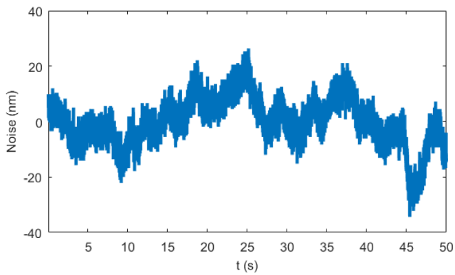
Figure 11. Closed-loop positioning noise (0.03Hz to 1MHz)
