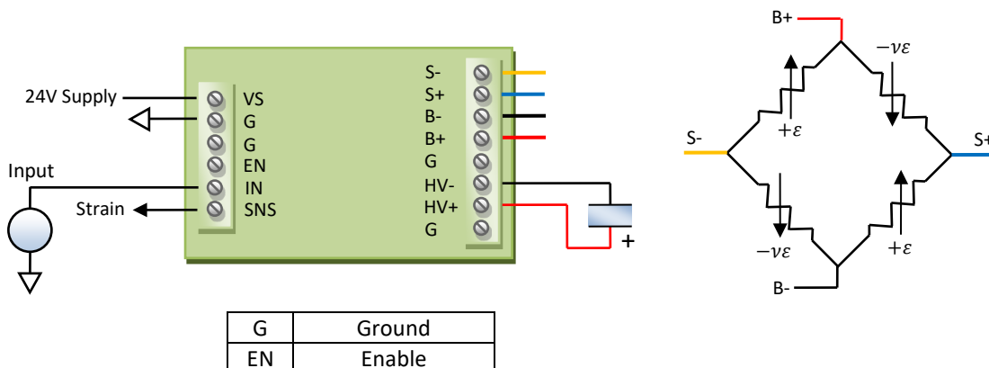
Figure 1. Basic Connection diagram
