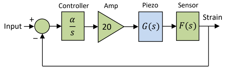
Figure 7. Feedback structure of the PDU150CL
