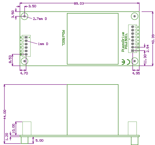
Figure 12. Dimensions (mm)
