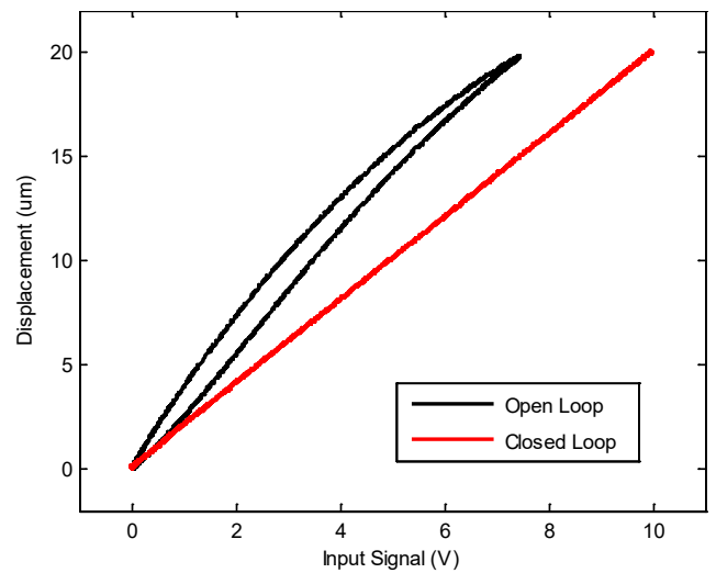
Figure 10. Open- and Closed-Loop response (1-Hz Sinusoid)
