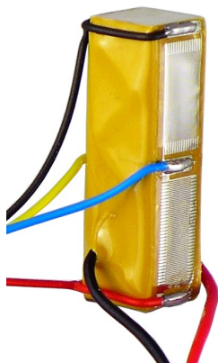
Figure 8. SCL050518 Actuator
