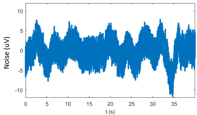
Figure 6. Total noise with a 350 Ohm Bridge (0.1Hz to 100Hz)
