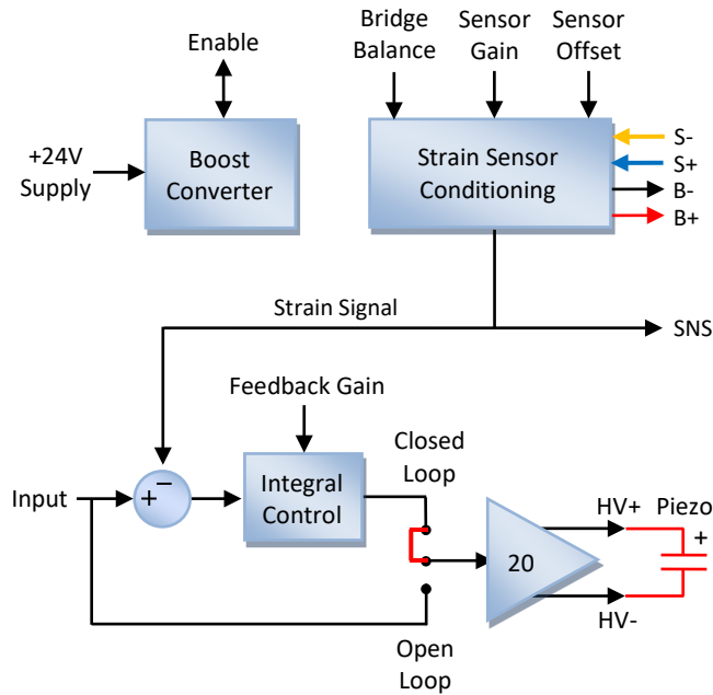
Figure 2. PDu150CL Block Diagram
