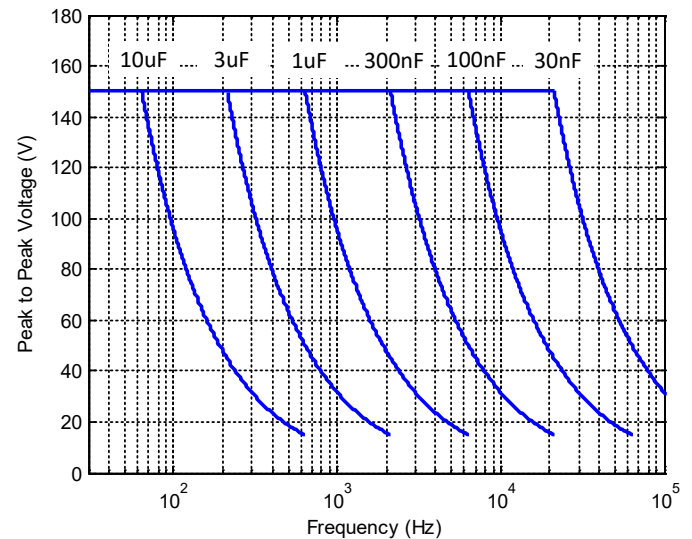
Figure 3. Power Bandwidth
