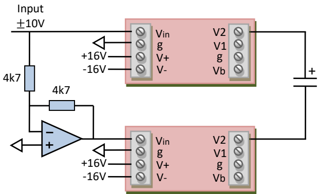
±400 V Piezo driver
