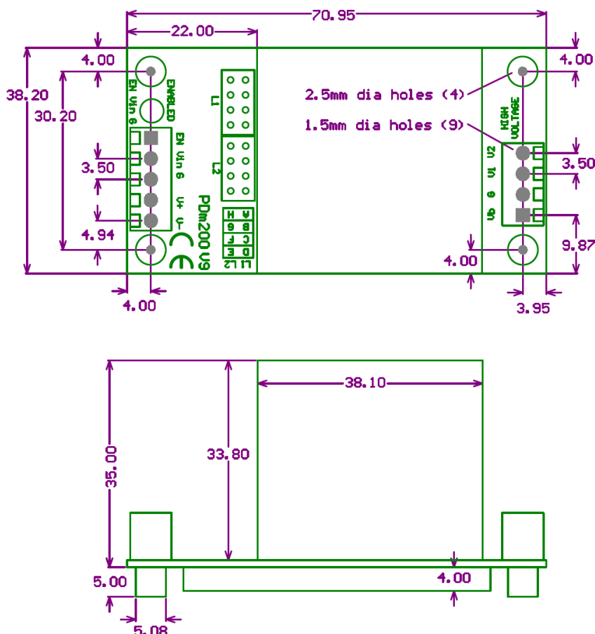
Figure 9. Dimensions (mm)
